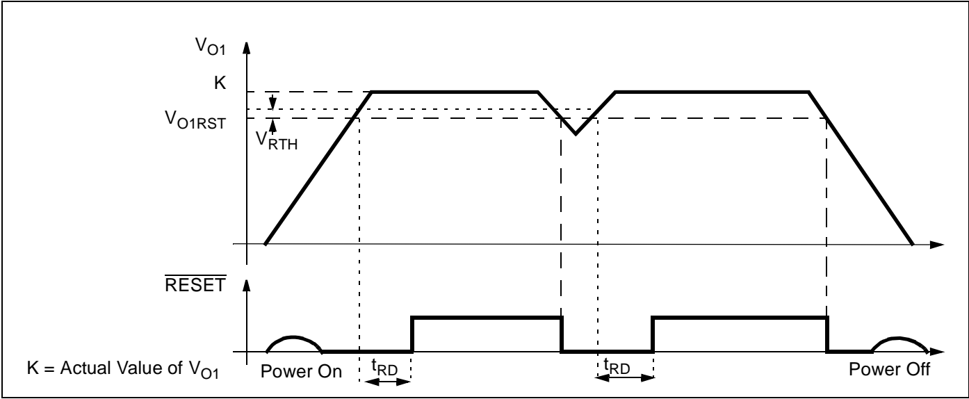
Figure 4: Internal Reset Voltages
