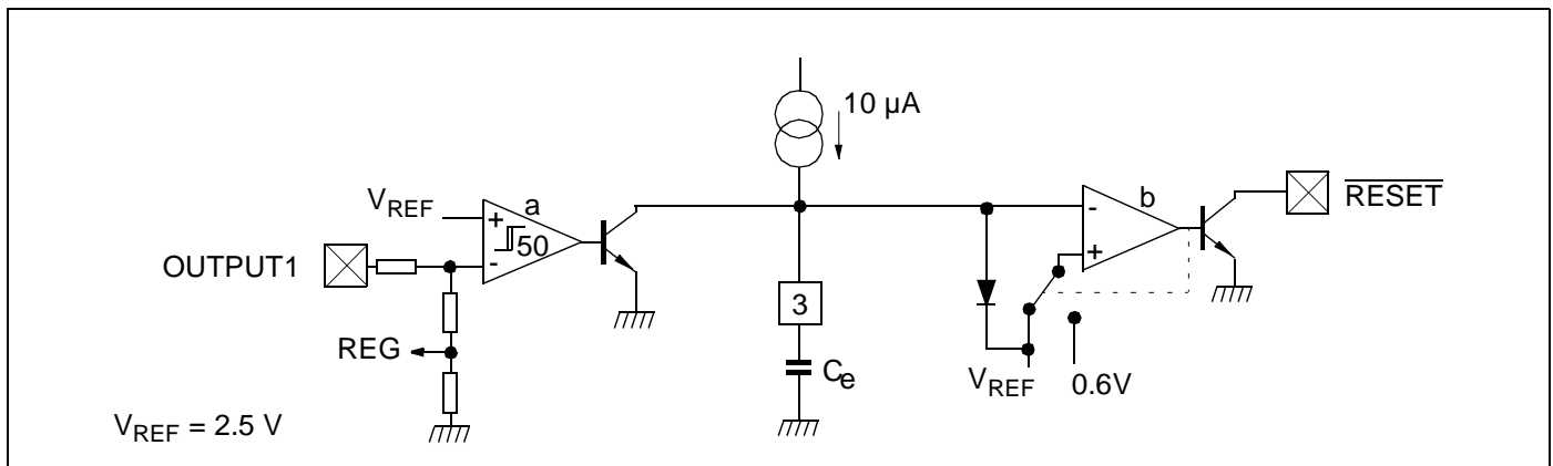
Figure 3: Reset Diagram
