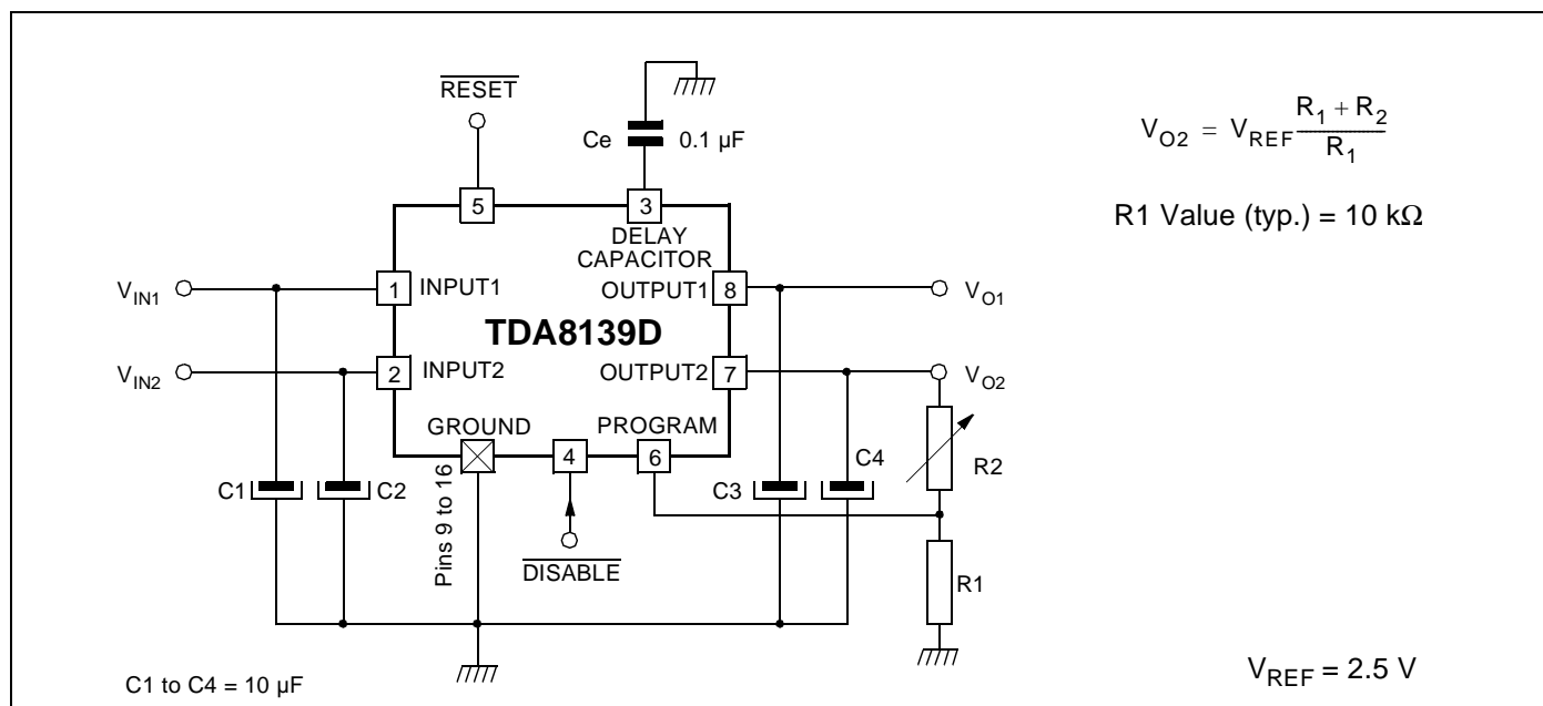
Figure 6: TDA8139D Typical Application
